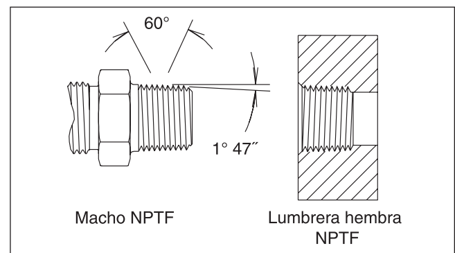
Fig. 1 – Rosca NPTF
